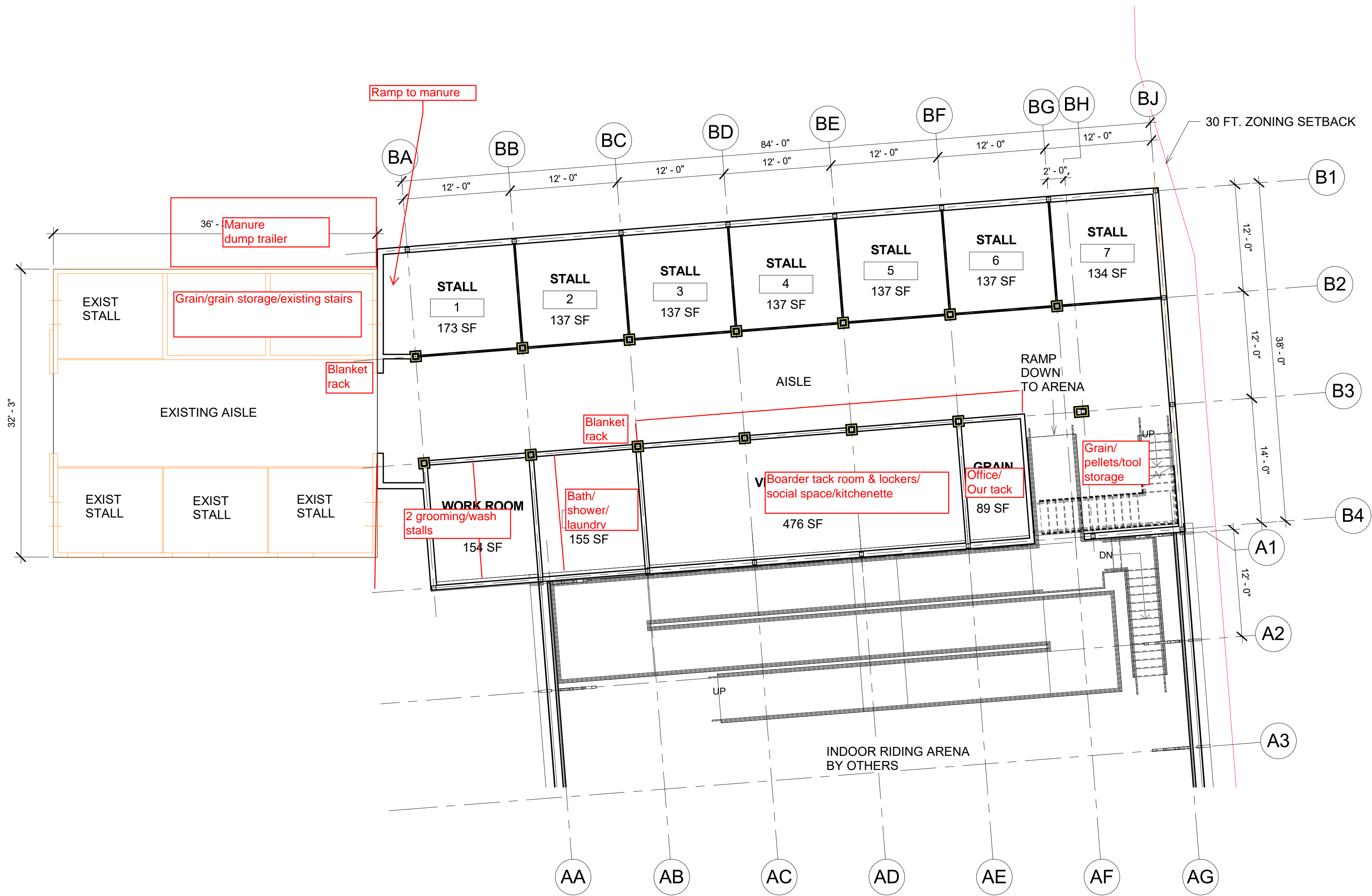
① BARN LEVEL 1 - ENLARGED 1/8" = 1'-0"
